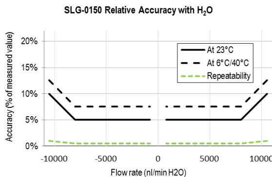
Figure 1: Flow meter accuracy and repeatability across the flow range. Relative error in % of measured value (left column) and absolute error in nl/min (right column) for H 2 O
