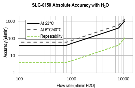
Figure 1: Flow meter accuracy and repeatability across the flow range. Relative error in % of measured value (left column) and absolute error in nl/min (right column) for H 2 O
